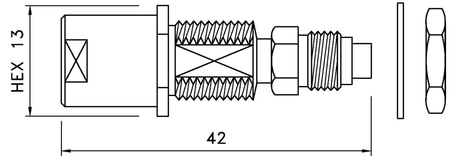
FME MALE TO FME FEMALE BULKHEAD
