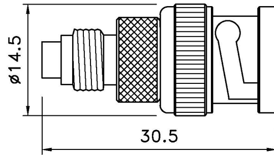
FME FEMALE TO BNC MALE
